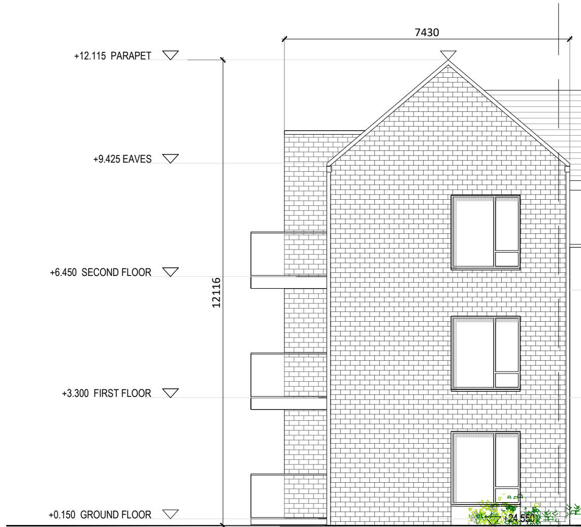
FRONT ELEVATION 1:100
