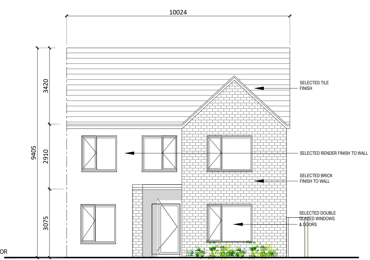
Front Elevation 1:100
