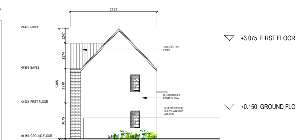
Side Elevation 1:200
