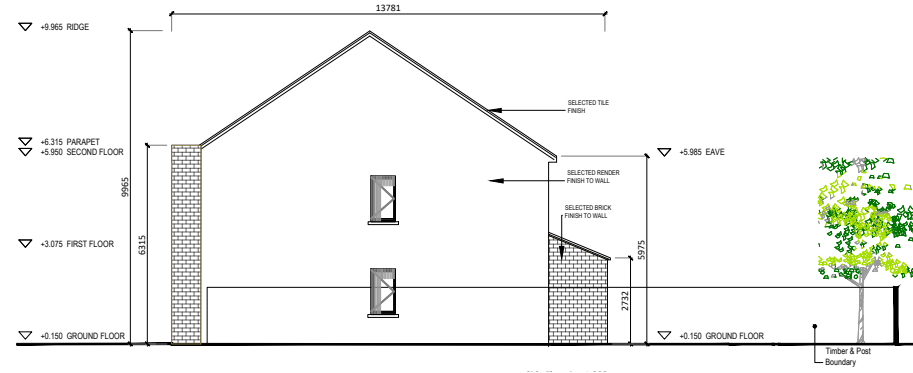
East/West Elevation 1:200
