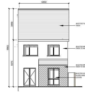
Rear Elevation 1:200
