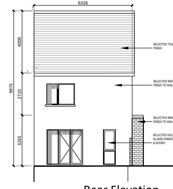
Rear Elevation 1:200
