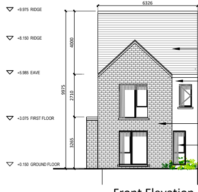
Front Elevation 1:200
